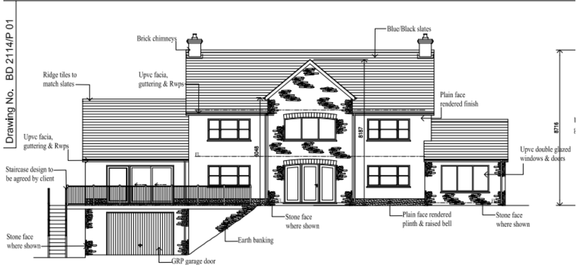
North Elevation 1:100th Scale
